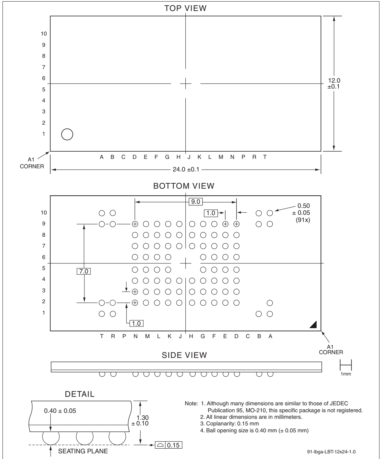
Figure 3: mini-NANDrive 91-Ball Low Profile Ball Grid Array (LBGA) SST Package Code: LBT
